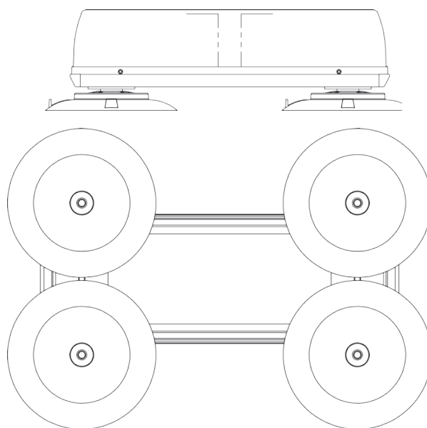
4 Point Magnetic/Vacuum Mounting (R1/R2 UK Specification)
